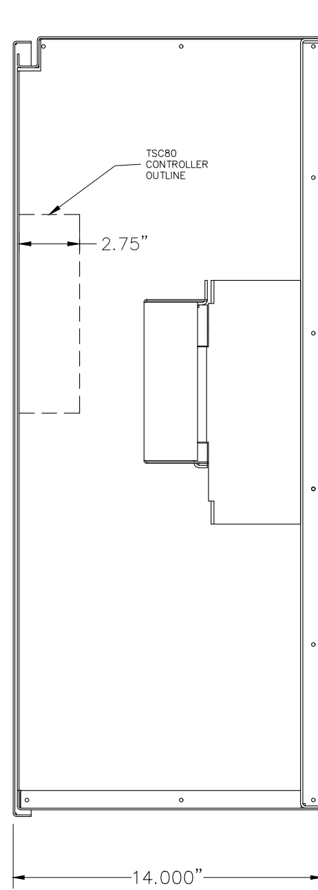
RHS VIEW
