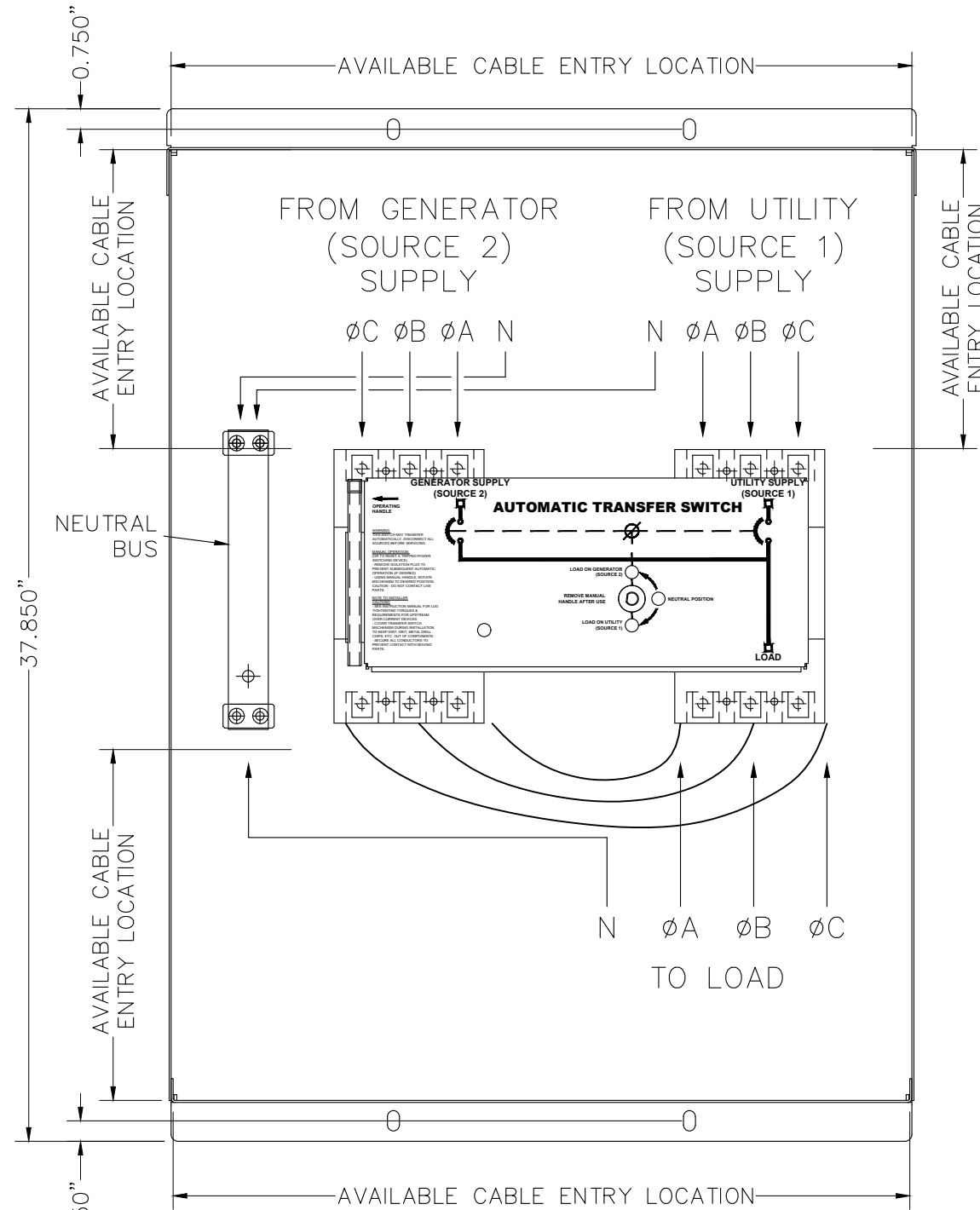
INTERIOR FRONT VIEW (DOOR NOT SHOWN)
